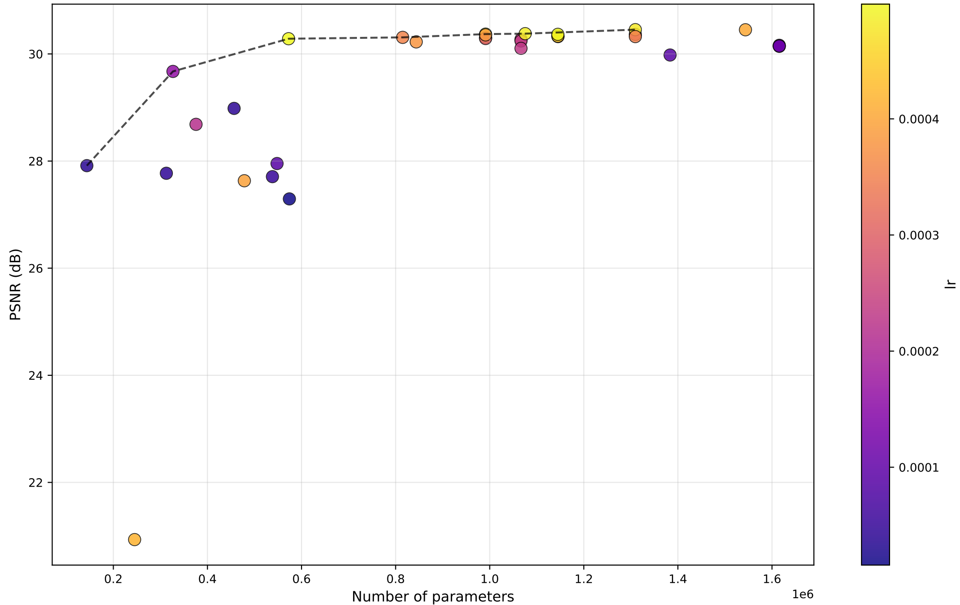
PSNR vs #Params — SRFormer — by l_r
